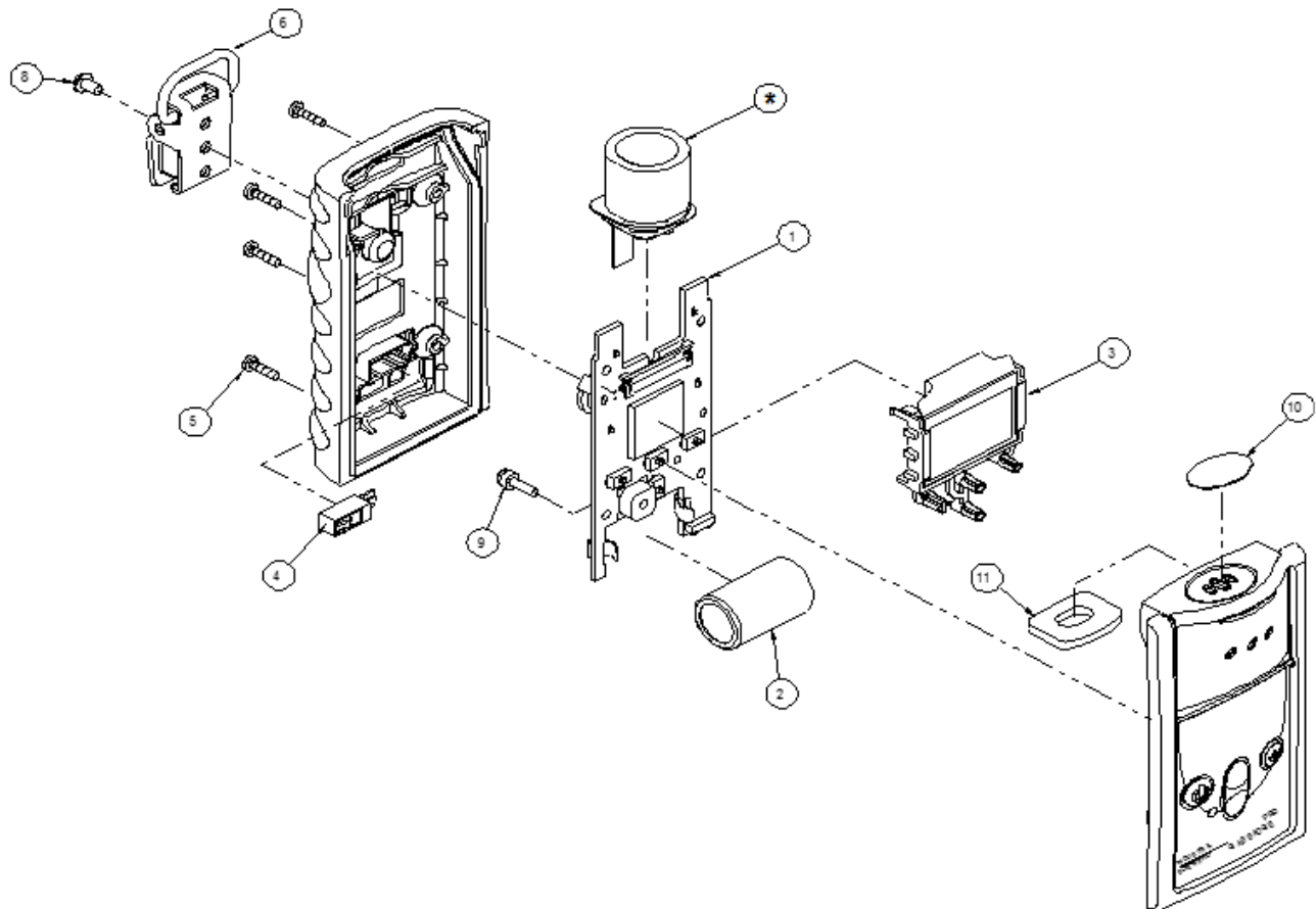
Detailed Components Drawing Showing Replacement Parts
