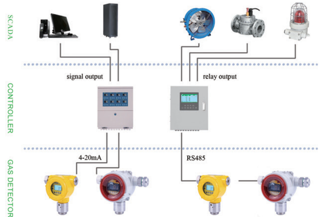
DIAGRAM of GAS DETECTION SYSTEM
