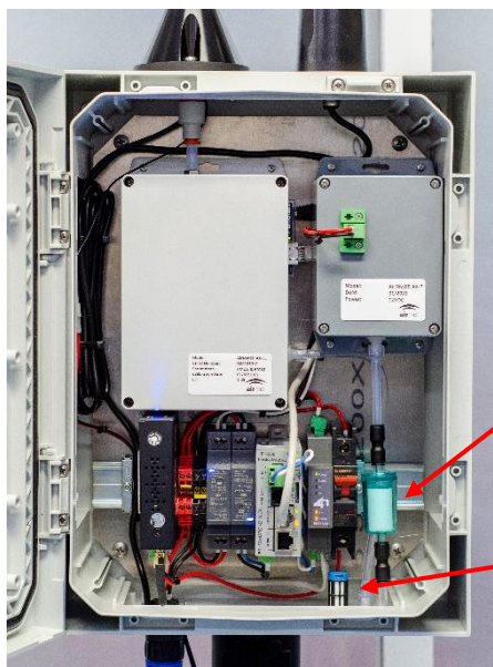
Figure 6.1 – Complete assembly
